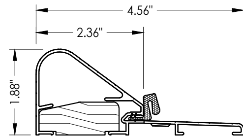
19 COASTAL OUTSWING THRESHOLD Wood / Aluminum Sill
