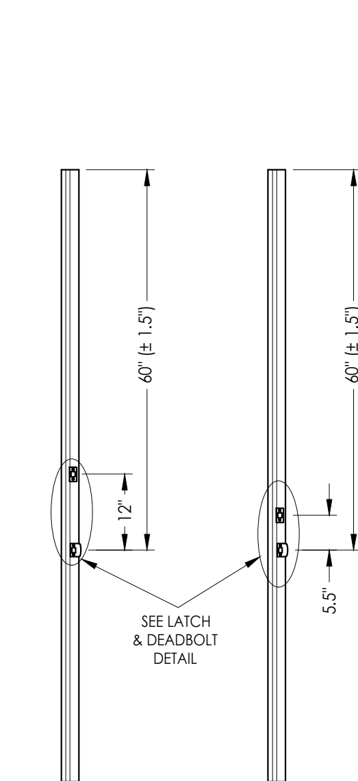
ASTRAGAL Latch & Deadbolt (12" o.c. spacing) ASTRAGAL Latch & Deadbolt (5-1/2" o.c. spacing)
