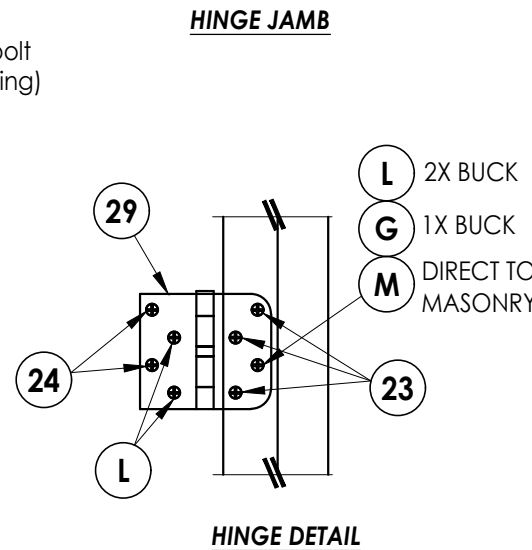
HINGE DETAIL
