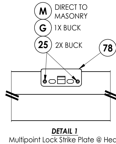
LATCH & DEADBOLT DETAIL Multipoint Lock
